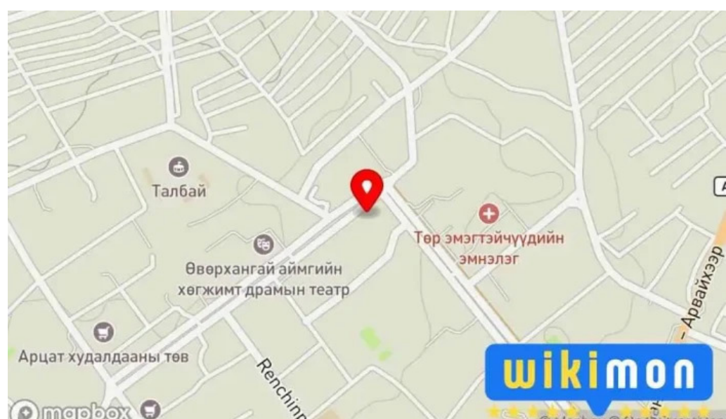
Gerel restaurant ?????? ??????
