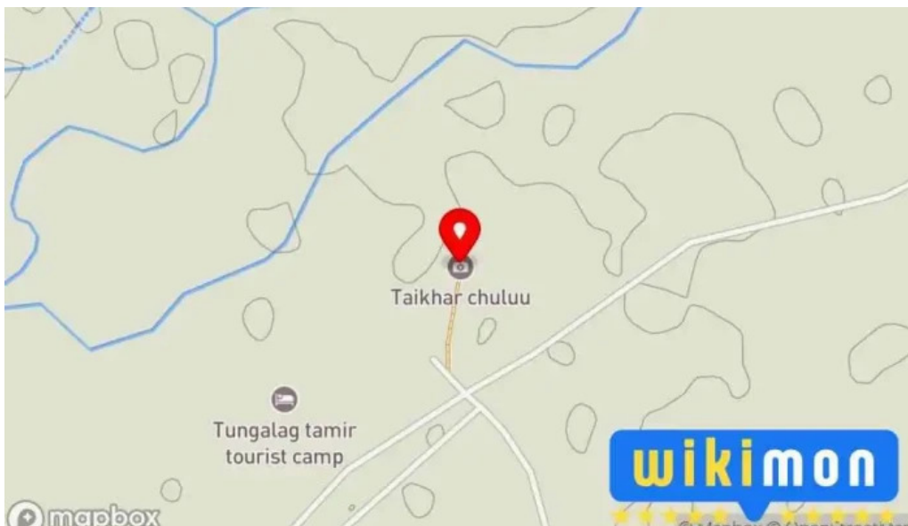
Taikhar rock ?????? ??????
