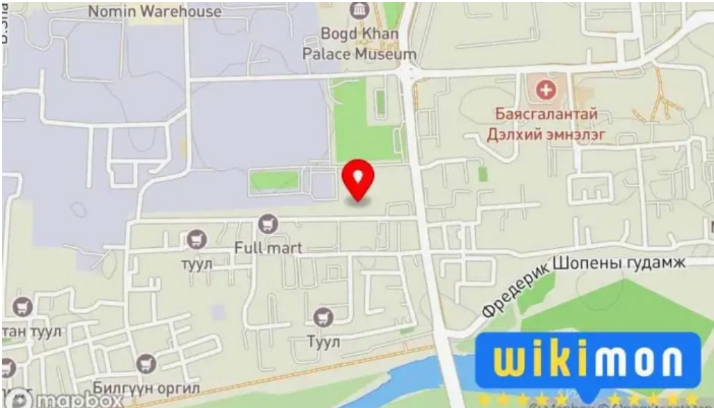
Agulah ??????? ??????
